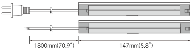
* LED Power Cord NDF3 40K-230V-C90-PC / OPC
