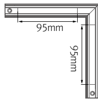
* 90 degree connector for NDF-EXL
