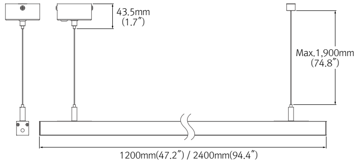
* NDF Extrusion Line
