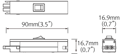
* NDF ON/OFF Switch
