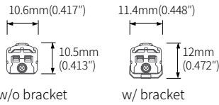
w/o bracket
