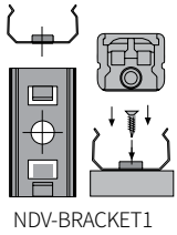
NDV-BRACKET1
