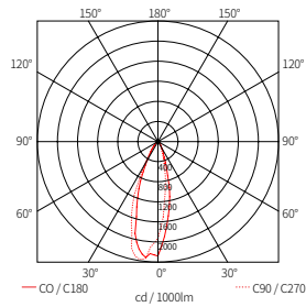
MCR-SP1 30K-24V-30-BK
